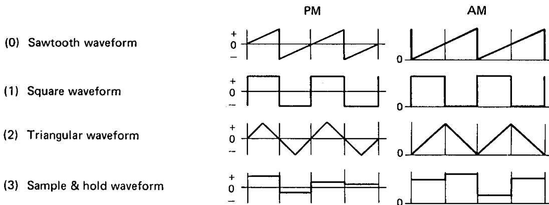
LFO WAVEFORMS
